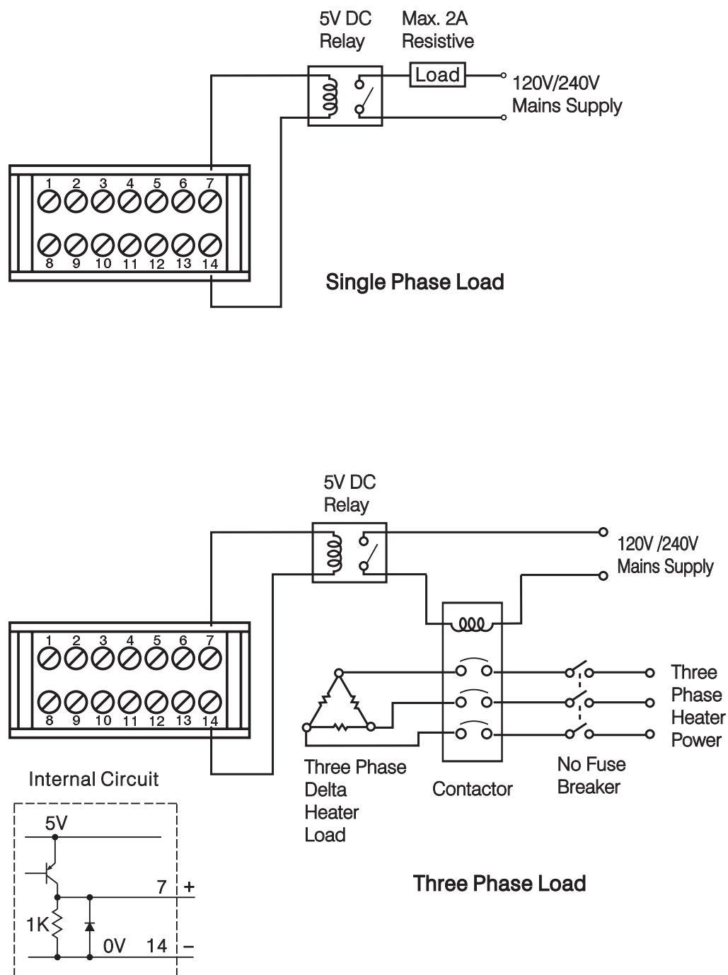
Figure 2.16 Alarm 1 Wiring
